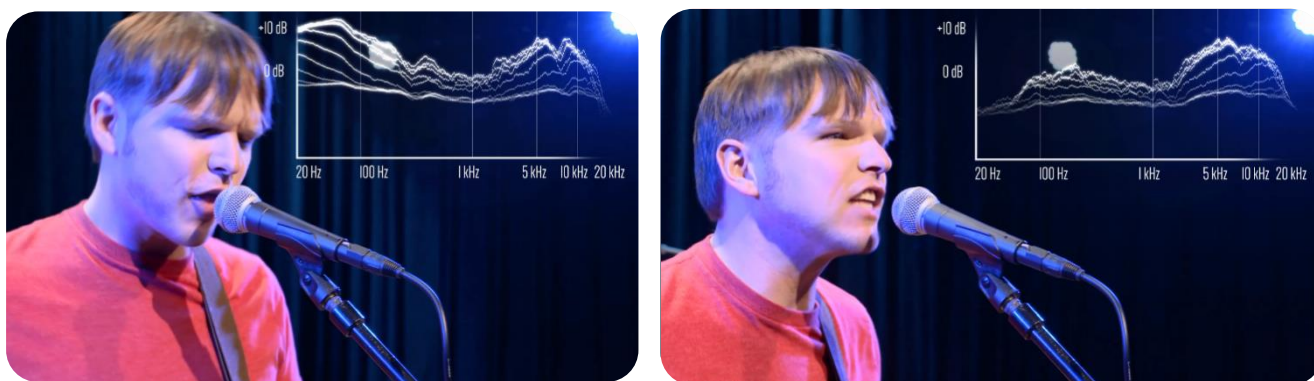
Simulated proximity effect response when a singer is directly on a directional microphone vs. slightly away. Notice the increase in bass response as the singer is closer to the microphone.
