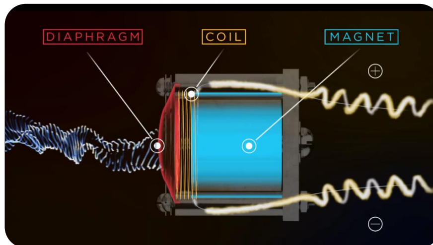
Major components and operation of a dynamic microphone when sound strikes the front of the diaphragm, on axis. Sound strikes the diaphragm and moves an attached coil within a magnetic field creating voltage across the coil.
